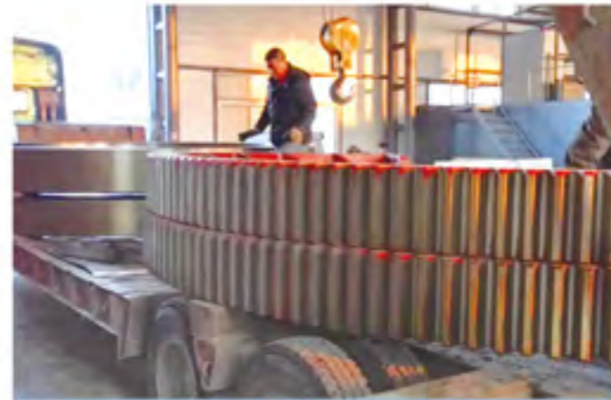
齿圈轮带/ Girth Gear Tyre \phi=5.4m
